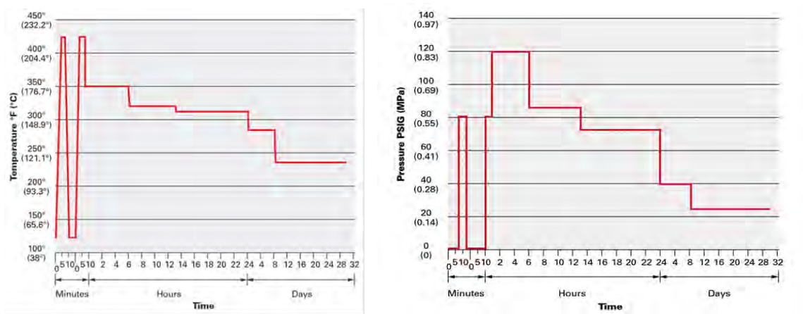
Figure. 7. Temperature and Pressure Profile used to qualify heat shrink Cable Accessories for use in Nuclear Power Plant Environments
